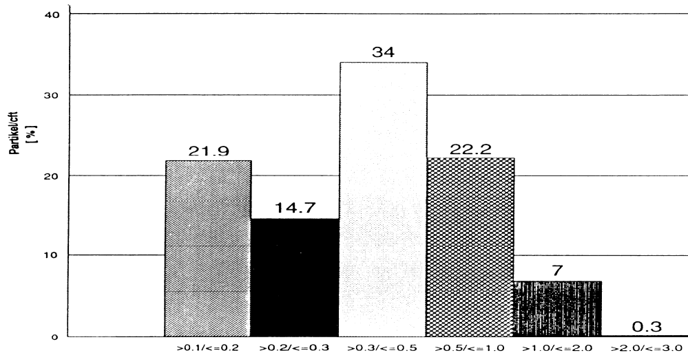
Fig. 2: Relative frequency of the Classes of Particle Size (size in μm)
